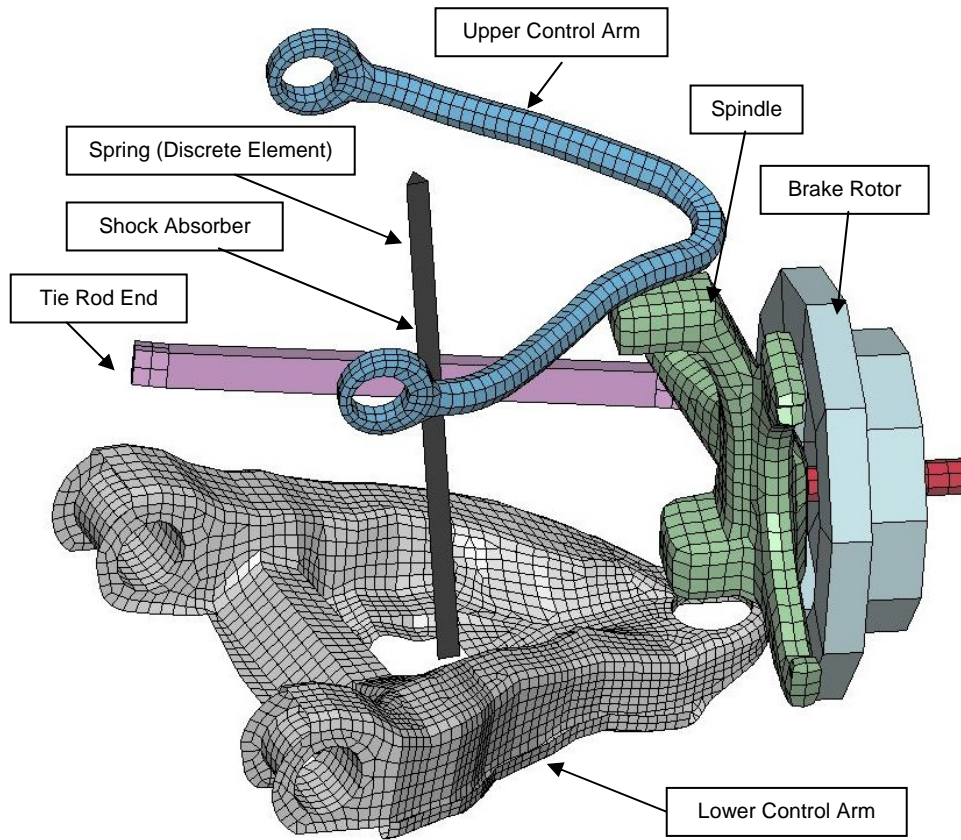
Figure 2. New Front Suspension Model Components
