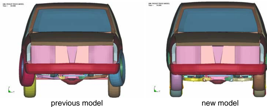
Figure 7. Improper Steering System Geometry Fixed
