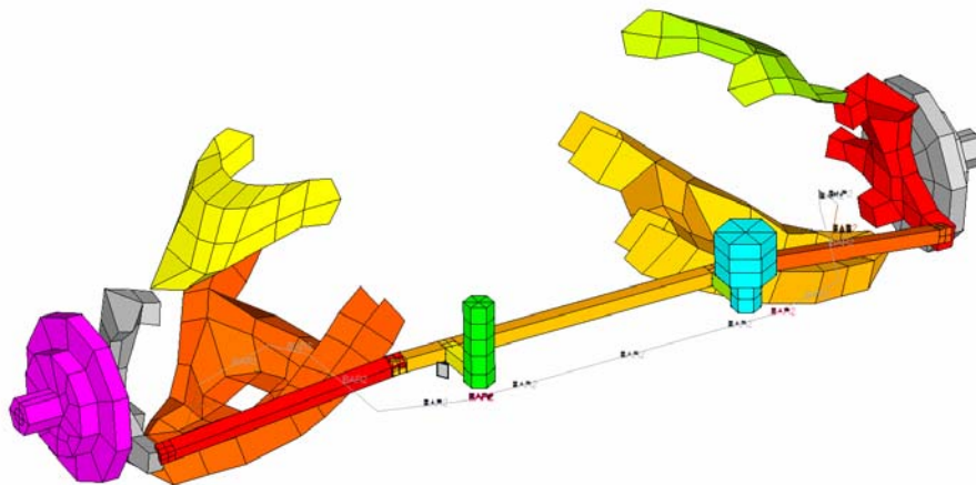
Figure 3. Old Front Suspension/Steering Subsystem Models
