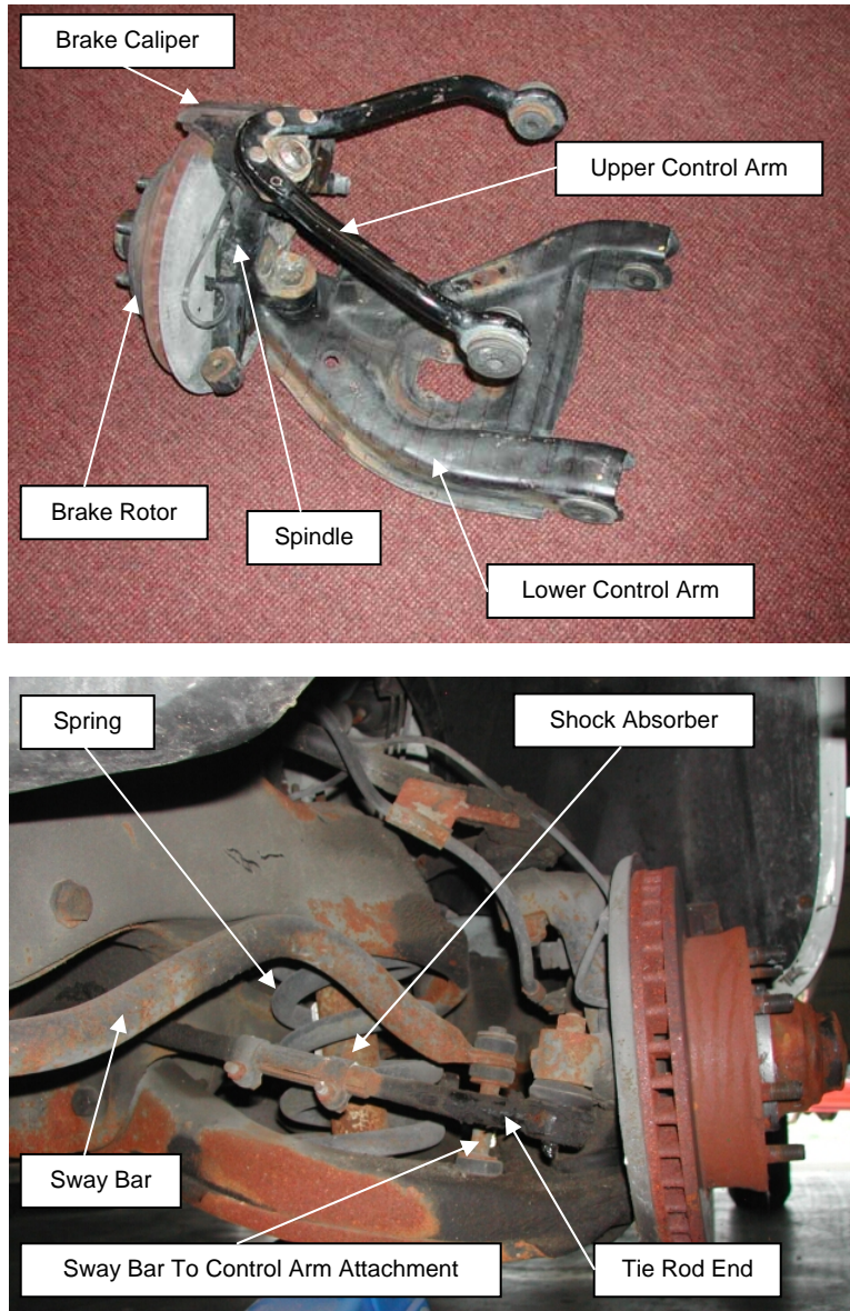
Figure 1. C2500 Front Suspension Components
