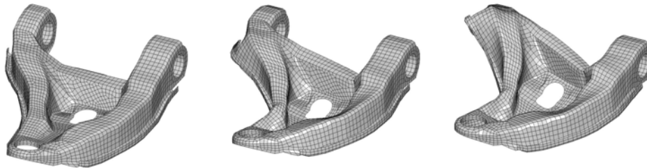
Figure 5. Lower Control Arm Deformation Simulation
