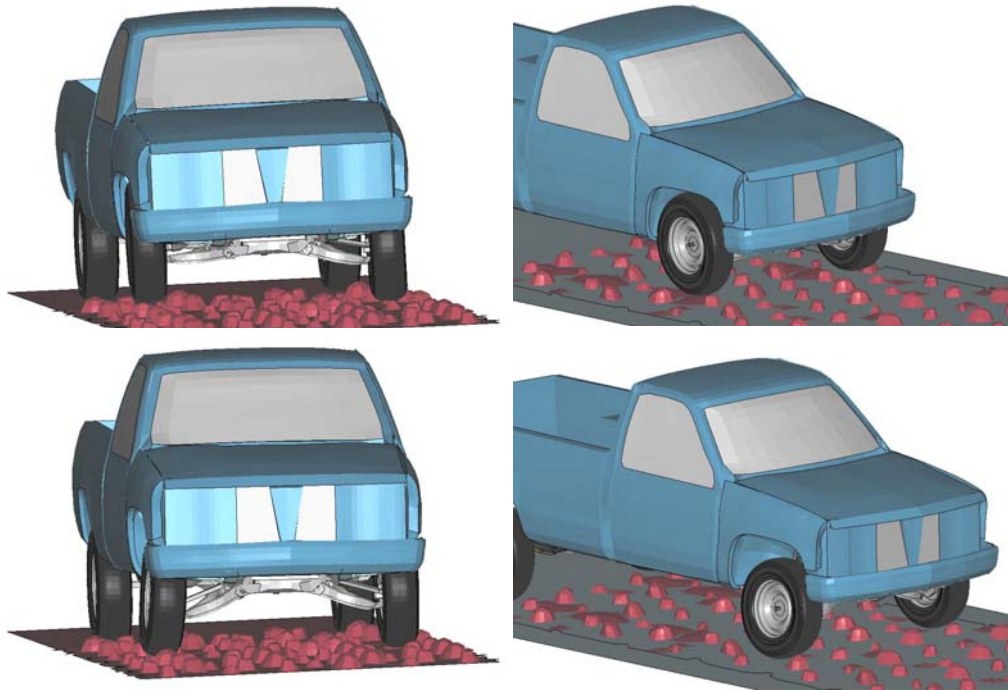
Figure 8. Rocky Ground Simulation Sequential Photos
